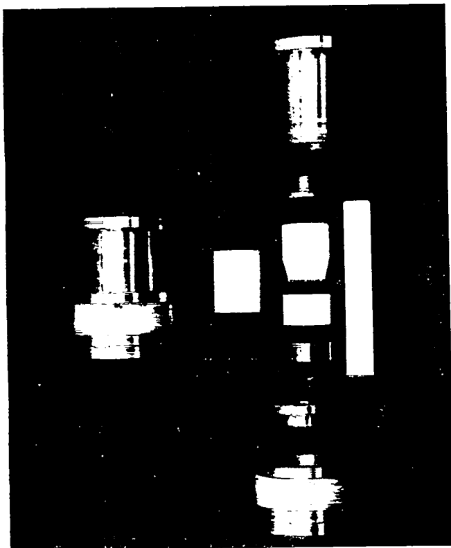
Fig. 1. High Temperature Acid Dissolution Bomb. with added advantages of capability to use HF as a solvent, (2) ease of handling, (3) reusable containers, and (4) quantitative containment of the sample in a container suitable for subsequent chemical treatments if desired.
